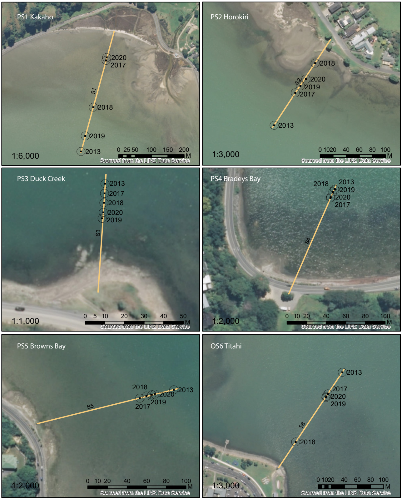
Fig. 5. Transects showing the distance from subtidal plates to where soft subtidal mud transitioned to firmer sediments closer to the shoreline (2013, 2017, 2018, 2019 and 2020).
