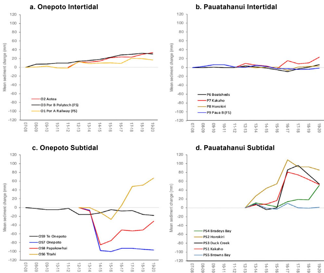
Fig. 2. Cumulative change in mean sediment level over buried plates at individual monitoring sites in Te Awarua-o-Porirua Harbour.
