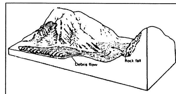
5. Debris flow
