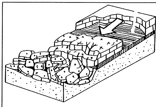
3. Planar slide
