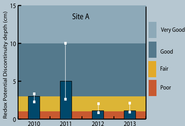
Figure 4. RPD depth (mean and range), Waikanae Estuary (2010-2013).
