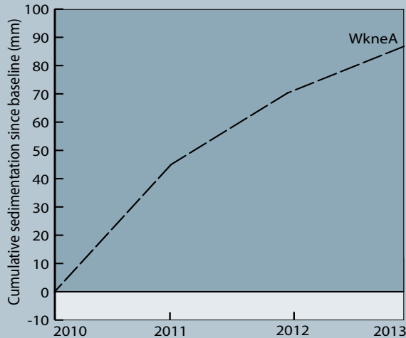
Figure 2. Cumulative change in sediment level from 2010-2013.
