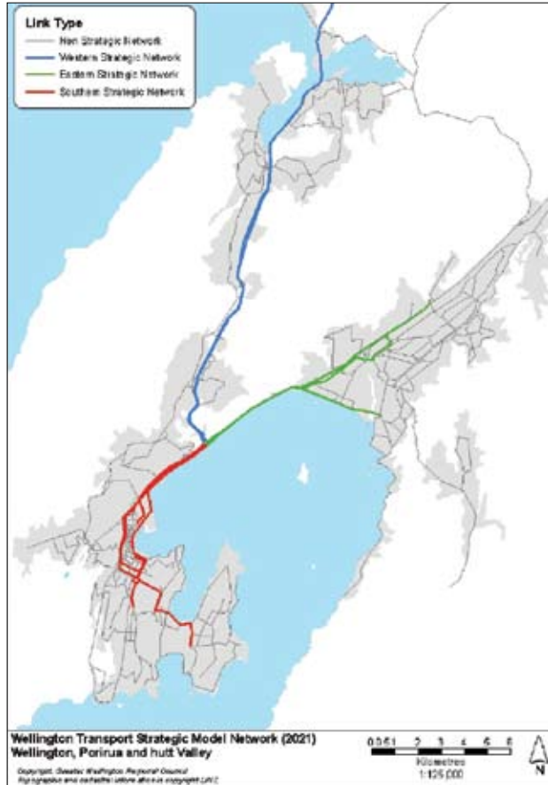
Figure 34: WTSM model network (2021), Wellington, Porirua and Hutt Valley. Source: GWRC
