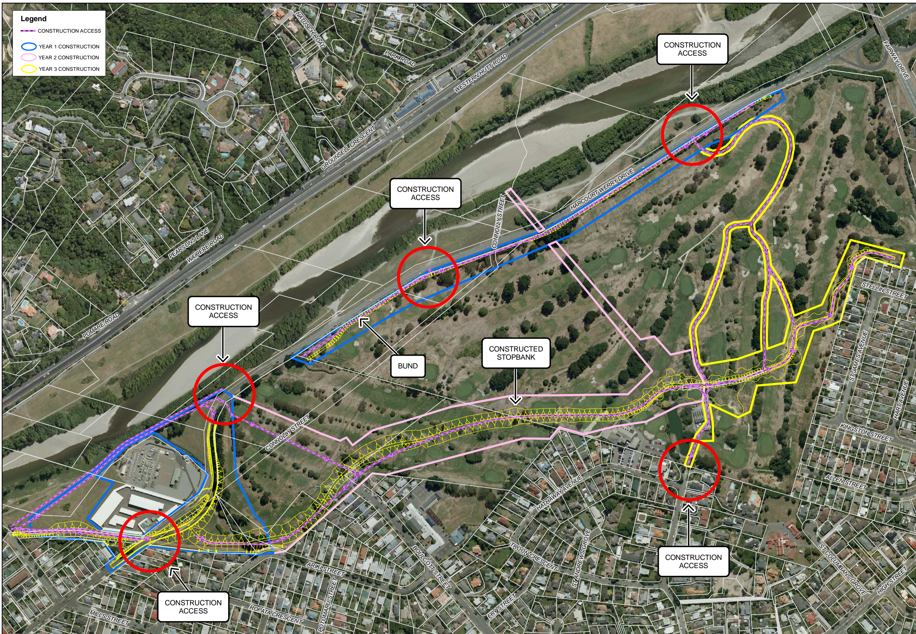
BOULCOTT / HUTT STOPBANK - Overall Layout
