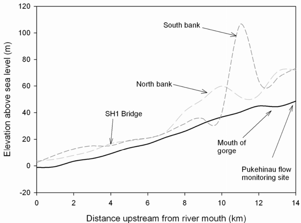
Figure 2.3: Longitudinal section of the Otaki River bed (bold black line) and bank profiles compiled from 1991 Greater Wellington survey data (note vertical exaggeration)
