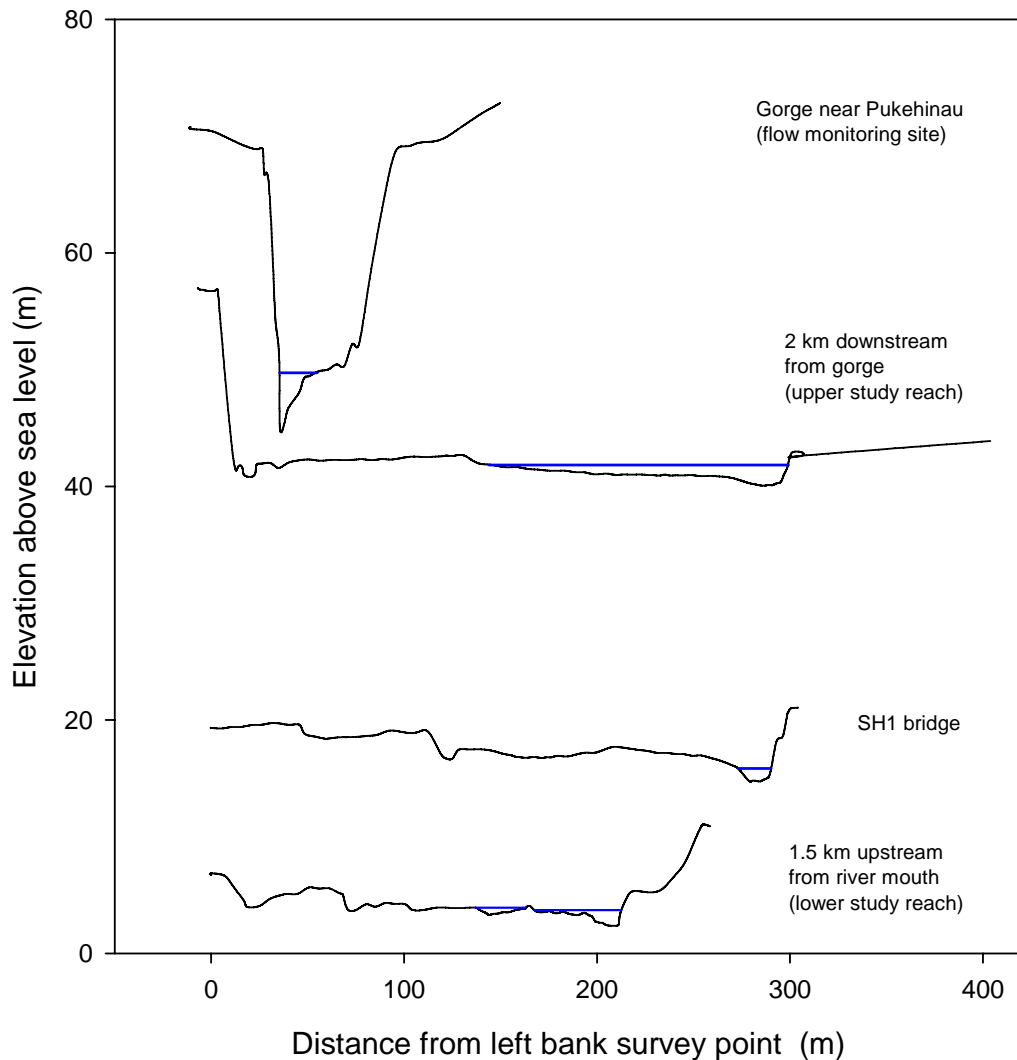
Figure 2.4: Selected Greater Wellington survey cross sections of the Otaki River channel from Pukehinau within the gorge (top section) to near the river mouth (bottom section). Elevation is metres above sea level and sections begin at the highest left bank survey point (note vertical exaggeration). Water levels on the date of survey (1 December 2005) are depicted by the blue lines.
