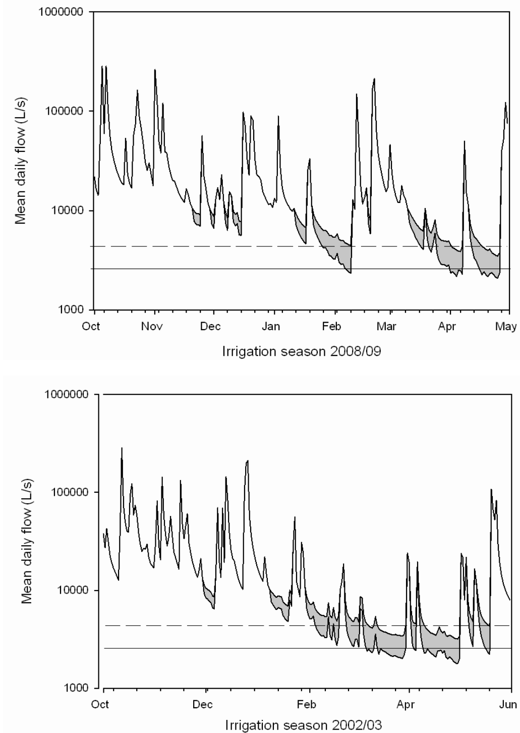
Figure 6.1: Mean daily flow for the Otaki River at Pukehinou through the irrigation season for an 'average' year (2008/09, top graph) and a 'dry' year (2002/03). Abstraction assuming a fully utilised existing core allocation of 2,120 L/s is modelled as the grey area beneath the hydrograph. The first restriction trigger flow of 4,375 L/s is shown as the horizontal dashed line (where abstraction is reduced to 1,800 L/s) and the recommended minimum flow of 2,550 L/s is the solid horizontal line. Note the log-scale on the y-axis of each graph.
