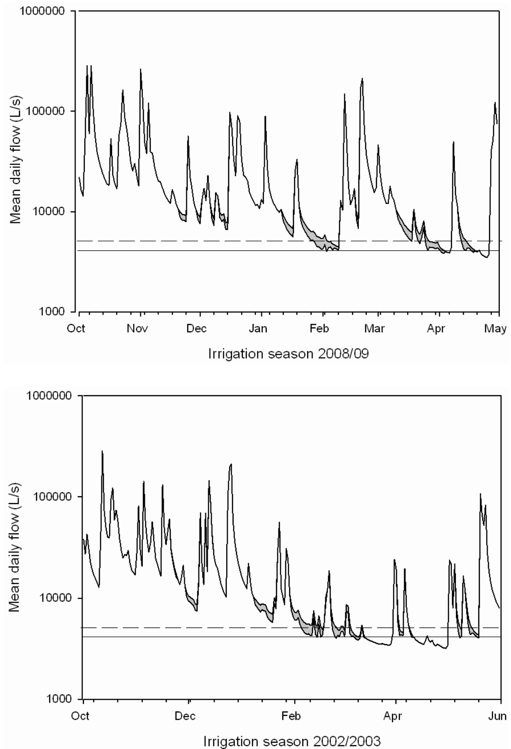
Figure 6.2: Mean daily flow for the Otaki River at Pukehinau through the irrigation season for an 'average' year (2008/09, top graph) and a 'dry' year (2002/03). Abstraction assuming a full prospective core allocation of 1,150 L/s is modelled as the grey area beneath the hydrograph. Nominal restriction trigger flow of 5,100 L/s is shown as the dashed horizontal line (where abstraction is reduced to 600 L/s) and the recommended minimum flow of 4,120 L/s is the solid horizontal line. Note the log-scale on the y-axis of each graph.
