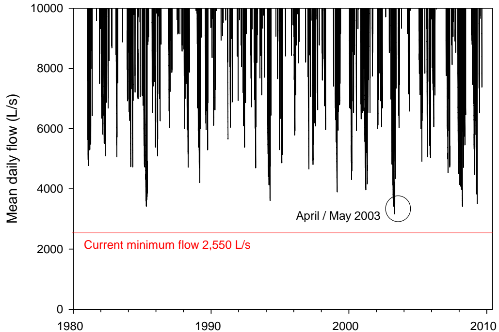
Figure 3.1: Mean daily flow for the Otaki River over 1980–2010 (only low flow portion of hydrograph shown)
