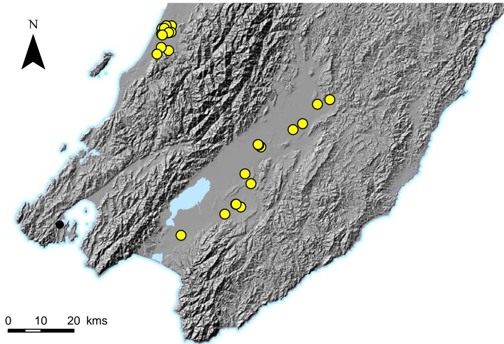
Figure 2.1: Greater Wellington's soil quality monitoring sites sampled in 2016/17
