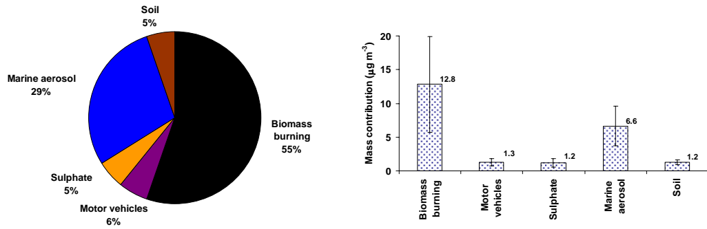
Figure 3.7: Relative source contributions to average PM 10 concentrations (left) and average mass contributions +/- one standard deviation (right)
