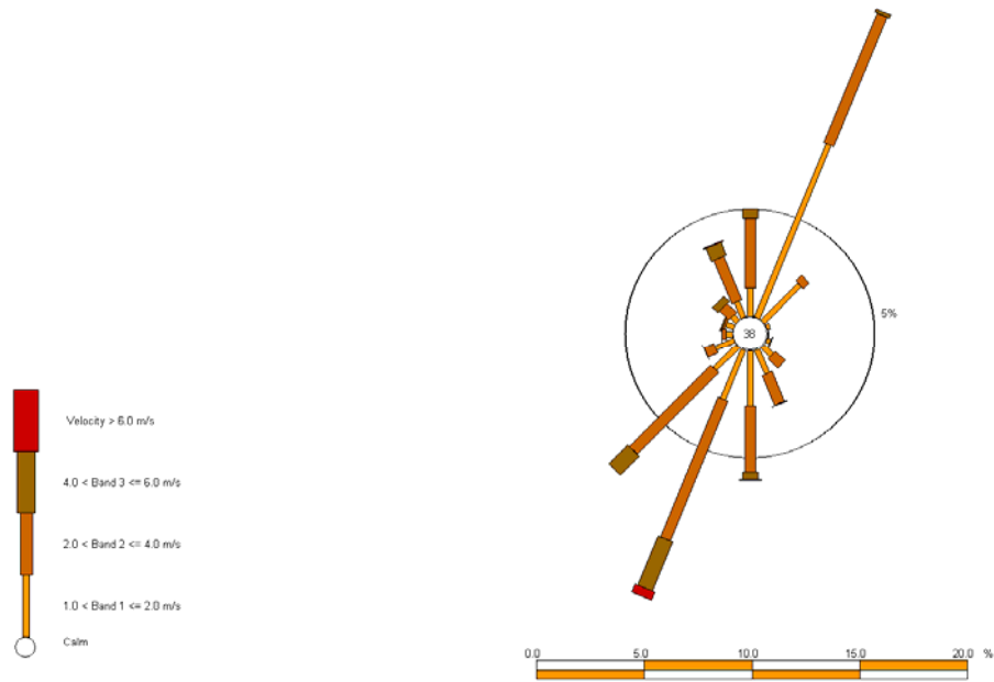
Figure 3.1: Wind rose for Glen Road, Raumati South for the period 1 June to 4 August 2010
